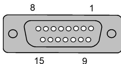
15-pin Sub-D, version DigIO
