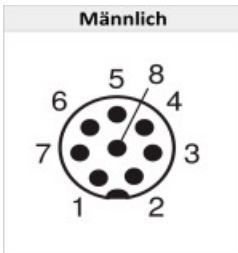
Figure 2: Contact configuration M12 plug
