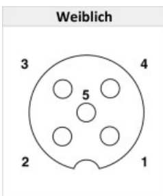
Figure 1: Contact configuration M12 socket
